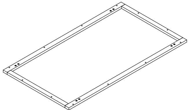
H: Base Frame (1pc)
