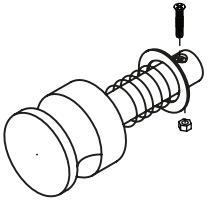
f: Swing lock (1pc)
